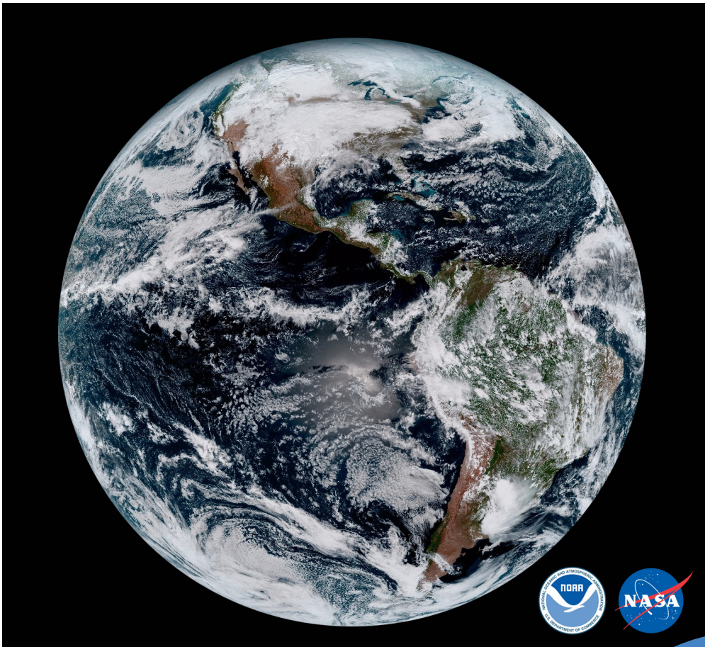
The Western Hemisphere taken by the ABI onboard the GOES-16.
